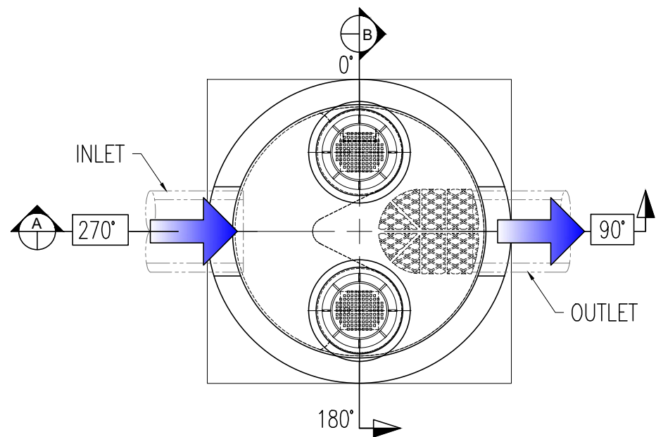
1 PLAN VIEW Scale: 3/16"
