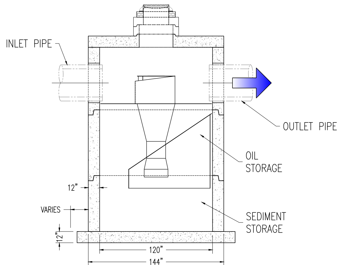
2 SECTION A Scale: 3/16"
