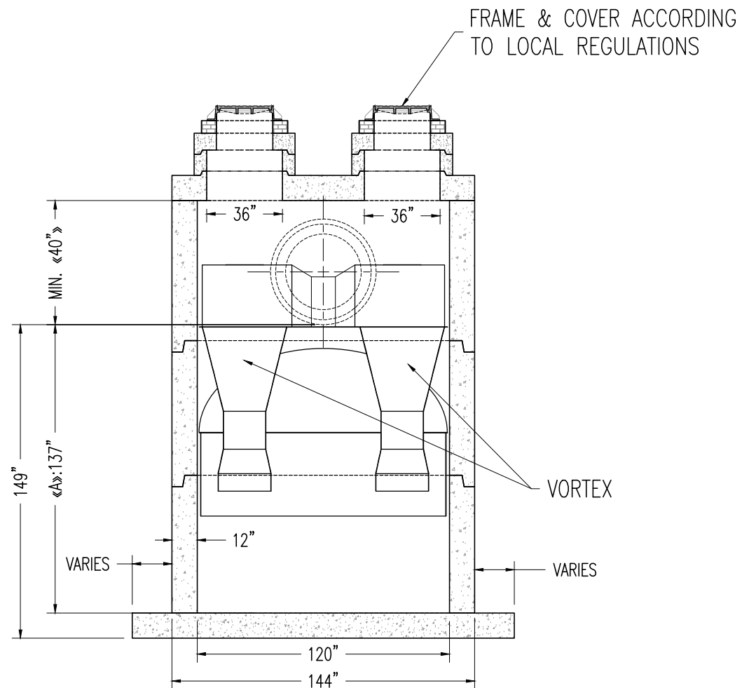
3 SECTION B Scale: 3/16"
