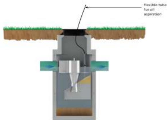
Figure 4: Oil cleaning
