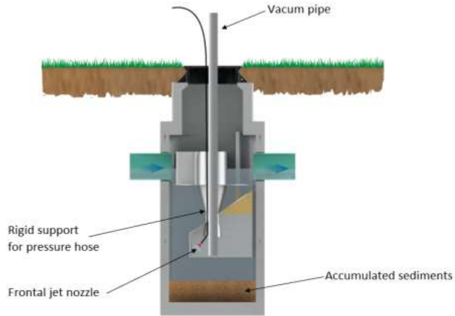
Figure 5 : Sediment cleaning
